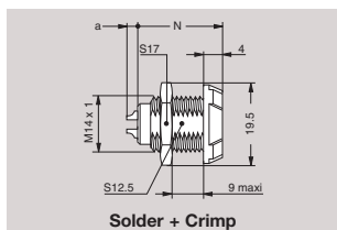
Solder + Crimp
